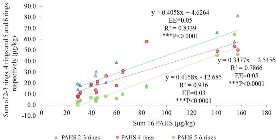
Figure 2. Performance of polycyclic aromatic hydrocarbons (PHHs) in the grass vs. the sum of PAHs of 2-3; 4; 5-6 rings.
